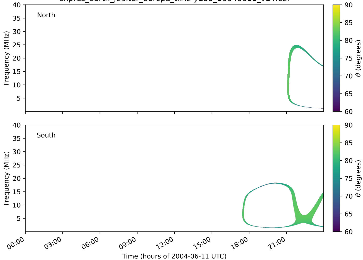
expres_earth_jupiter_europa_txka-y235_20040611_v14.cdf
