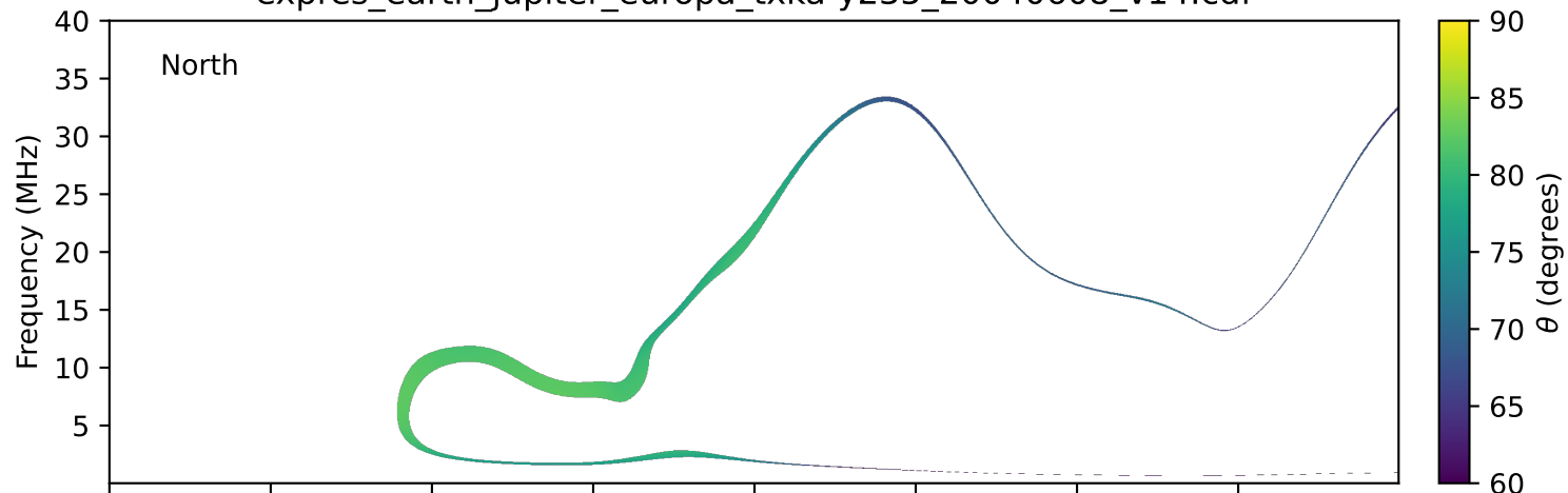
expres_earth_jupiter_europa_txka-y235_20040608_v14.cdf
