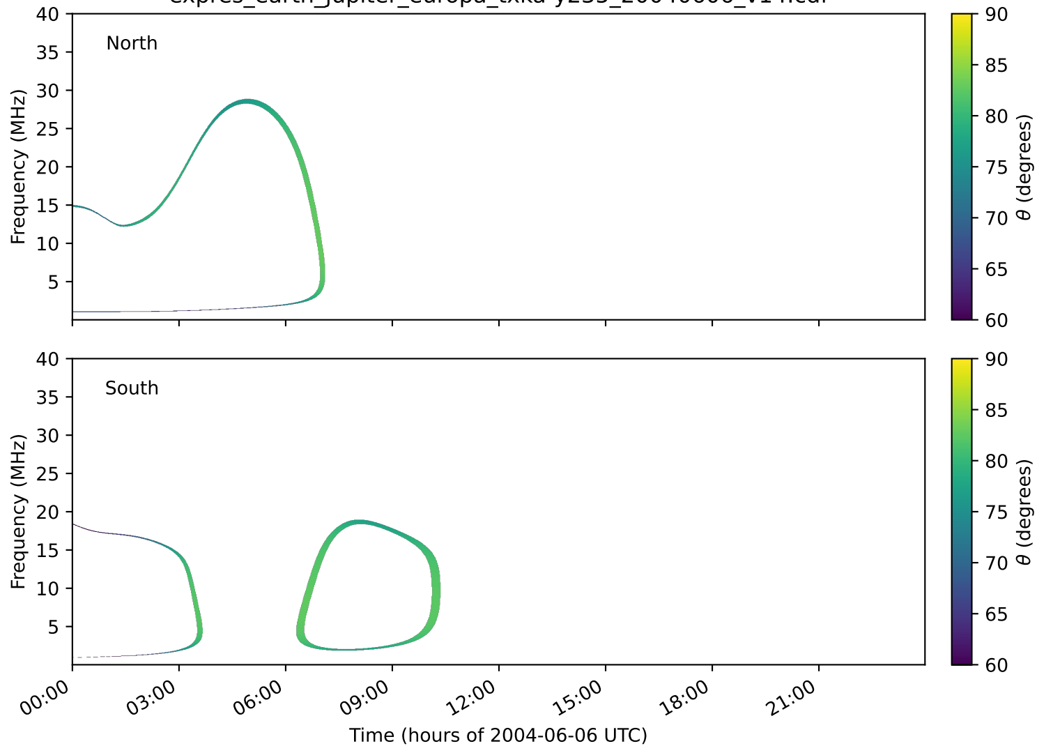
expres_earth_jupiter_europa_txka-y235_20040606_v14.cdf
