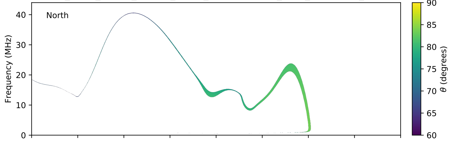
expres_earth_jupiter_europa_jrm09_lossc-wid1deg_3kev_20040627_v11.cdf
