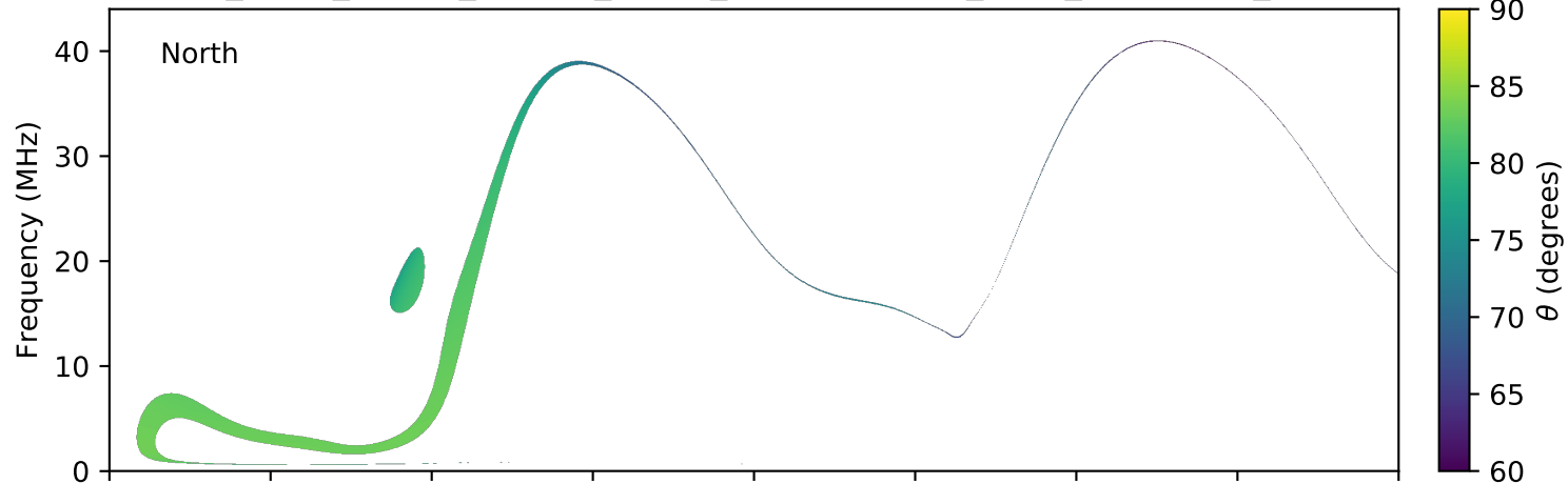
expres_earth_jupiter_europa_jrm09_lossc-wid1deg_3kev_20040626_v11.cdf
