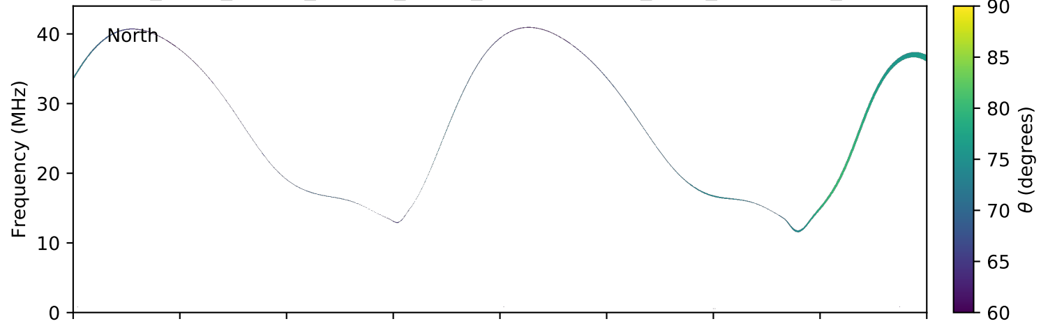
expres_earth_jupiter_europa_jrm09_lossc-wid1deg_3kev_20040623_v11.cdf
