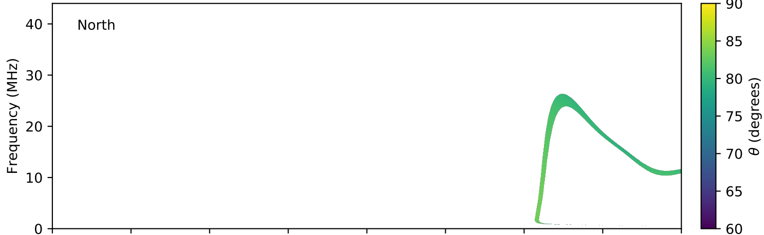
expres_earth_jupiter_europa_jrm09_lossc-wid1deg_3kev_20040620_v11.cdf
