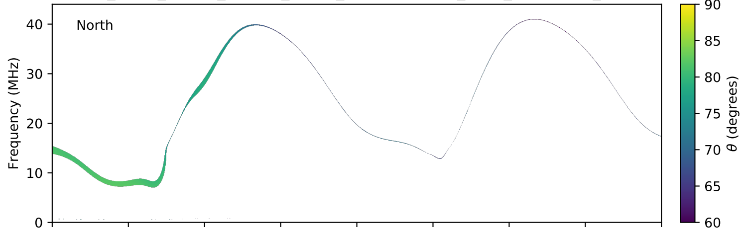
expres_earth_jupiter_europa_jrm09_lossc-wid1deg_3kev_20040619_v11.cdf
