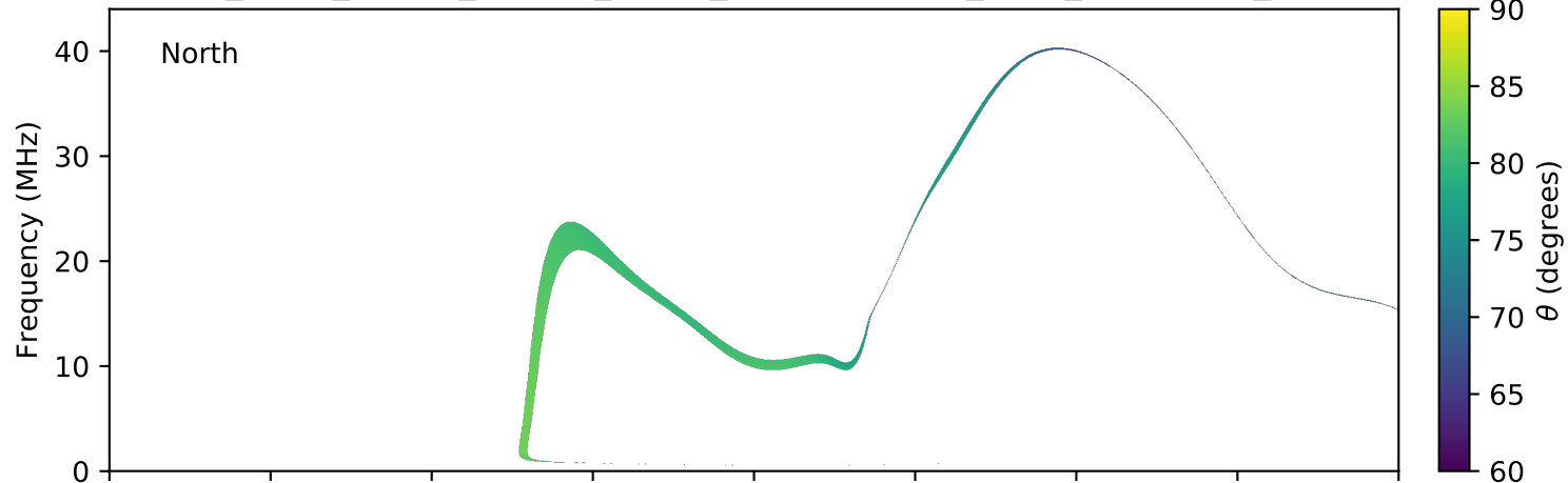
expres_earth_jupiter_europa_jrm09_lossc-wid1deg_3kev_20040606_v11.cdf
