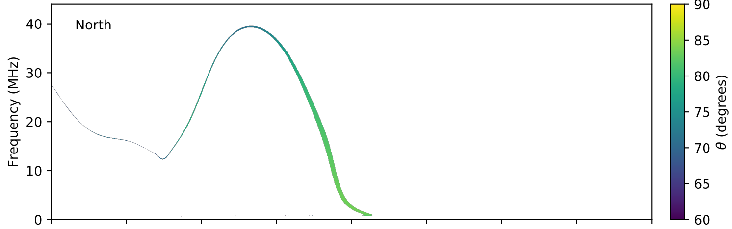
expres_earth_jupiter_europa_jrm09_lossc-wid1deg_3kev_20040604_v11.cdf
