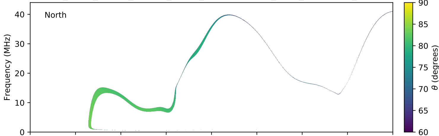
expres_earth_jupiter_europa_jrm09_lossc-wid1deg_3kev_20040601_v11.cdf
