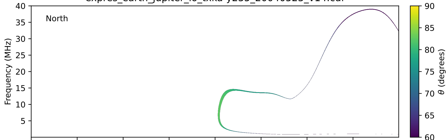
expres_earth_jupiter_io_txka-y235_20040523_v14.cdf
