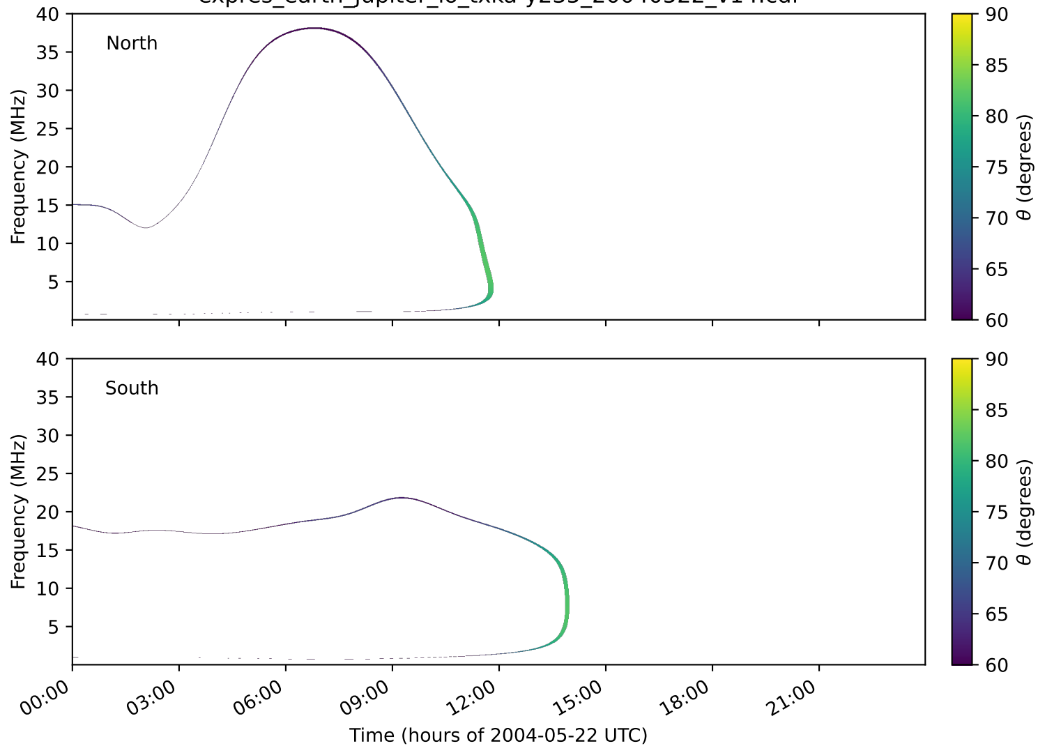
expres_earth_jupiter_io_txka-y235_20040522_v14.cdf
