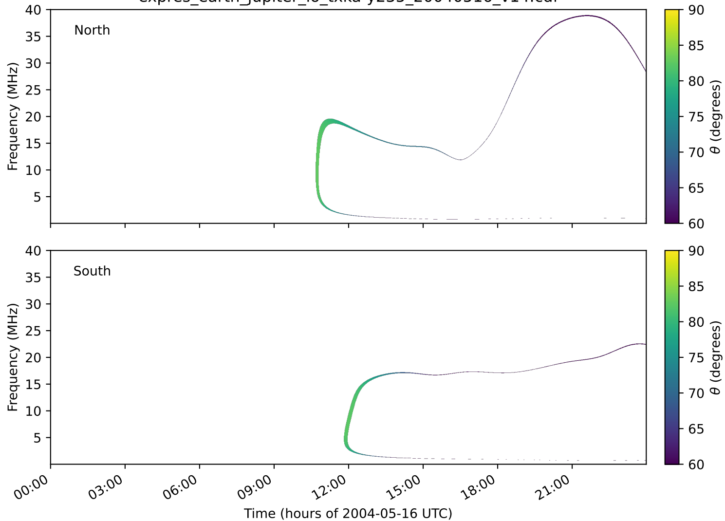
expres_earth_jupiter_io_txka-y235_20040516_v14.cdf
