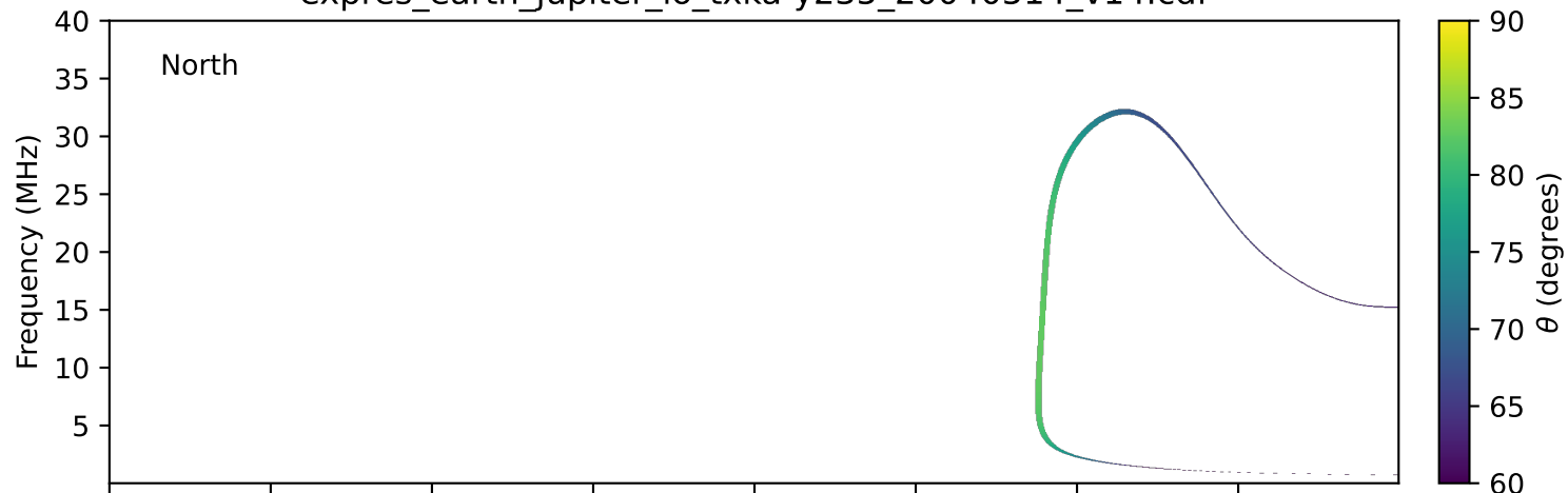
expres_earth_jupiter_io_txka-y235_20040514_v14.cdf
