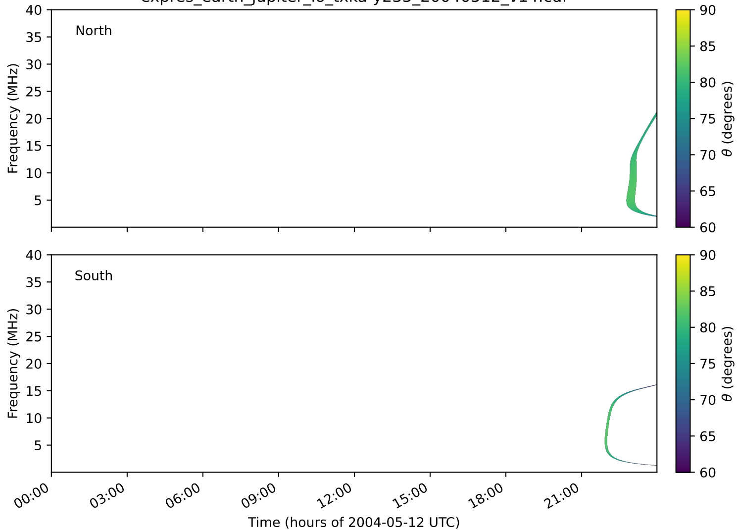
expres_earth_jupiter_io_txka-y235_20040512_v14.cdf
