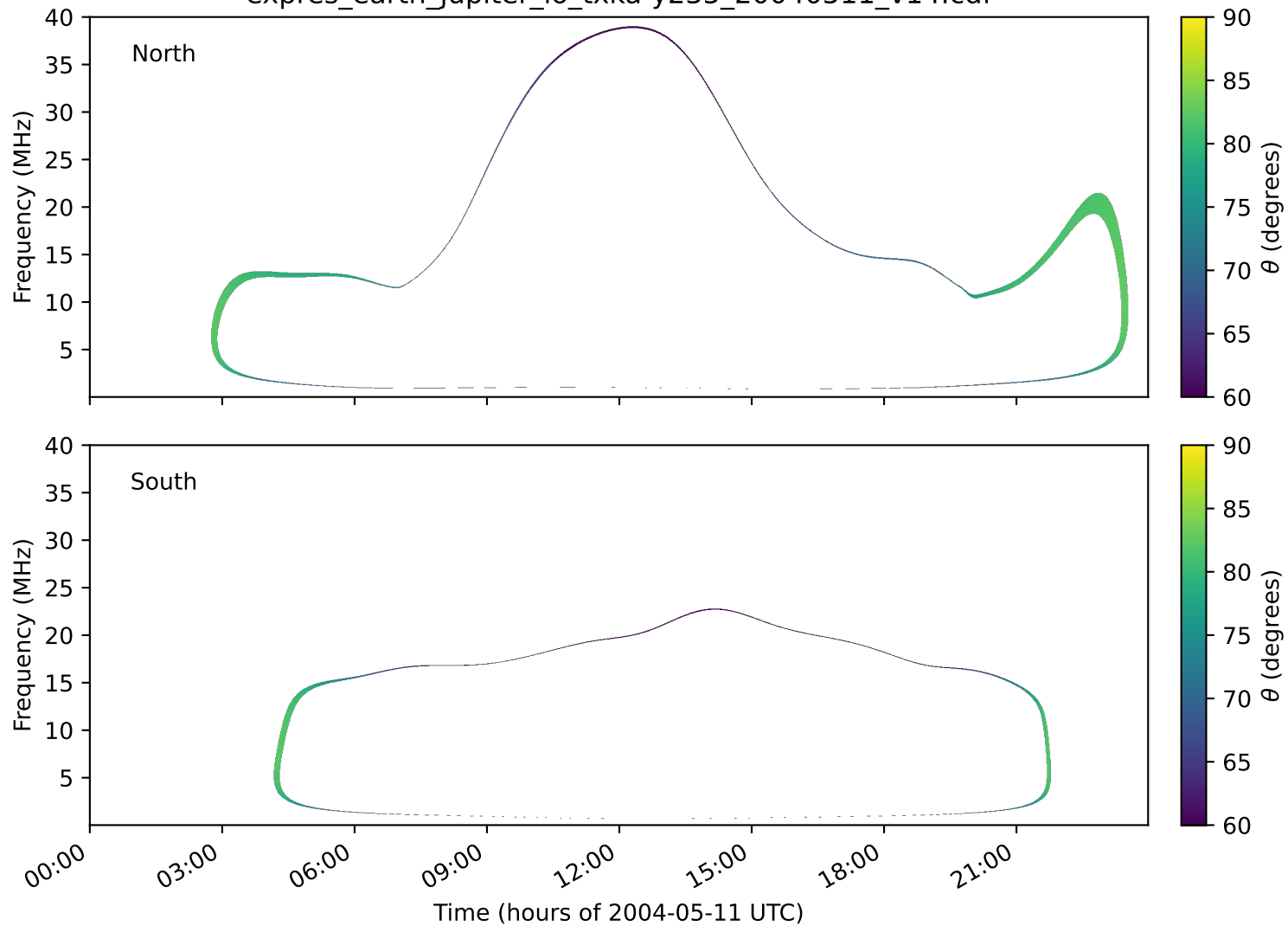
expres_earth_jupiter_io_txka-y235_20040511_v14.cdf
