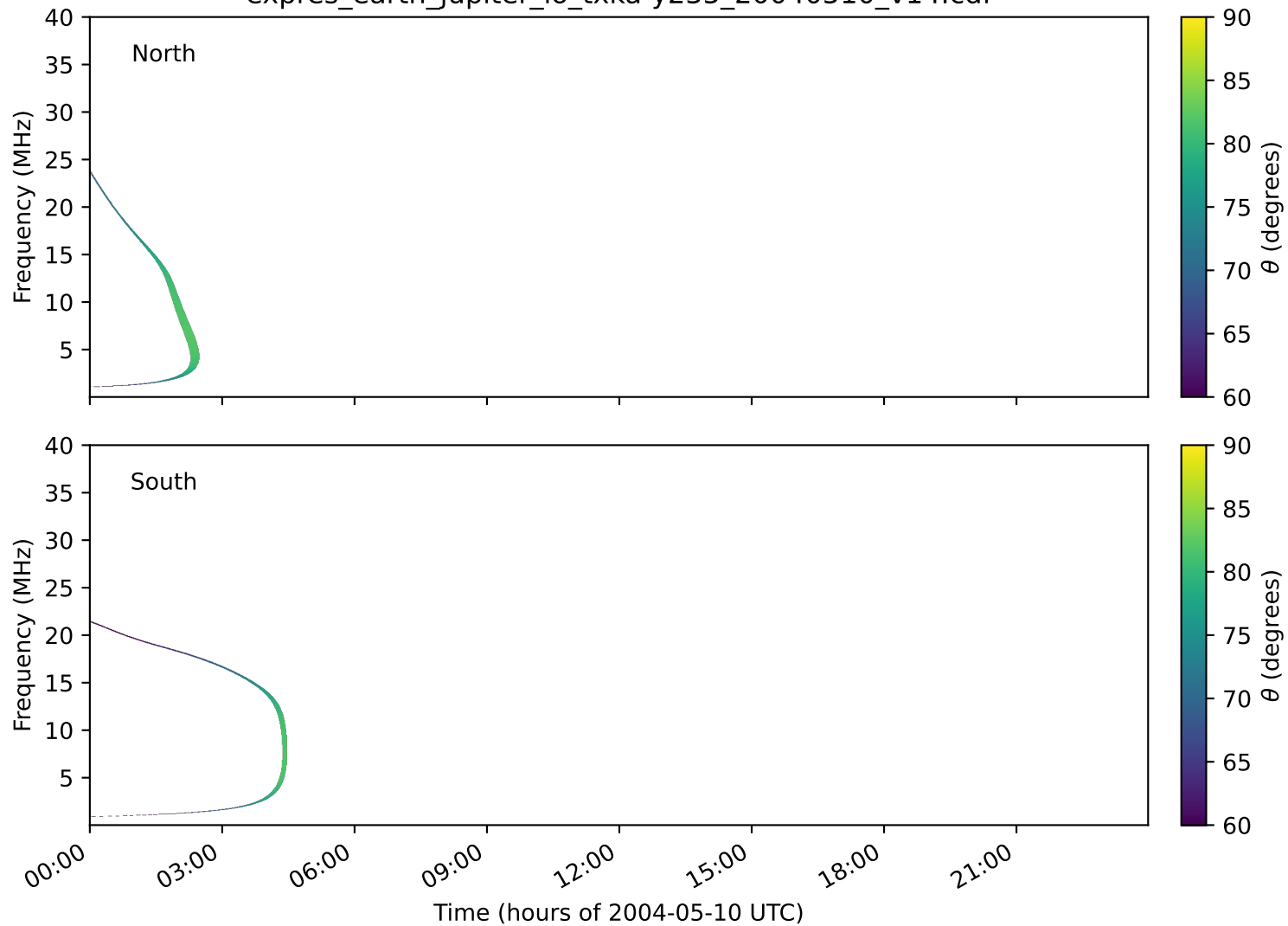
expres_earth_jupiter_io_txka-y235_20040510_v14.cdf
