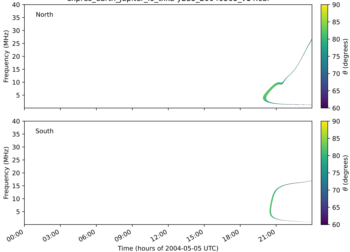
expres_earth_jupiter_io_txka-y235_20040505_v14.cdf
