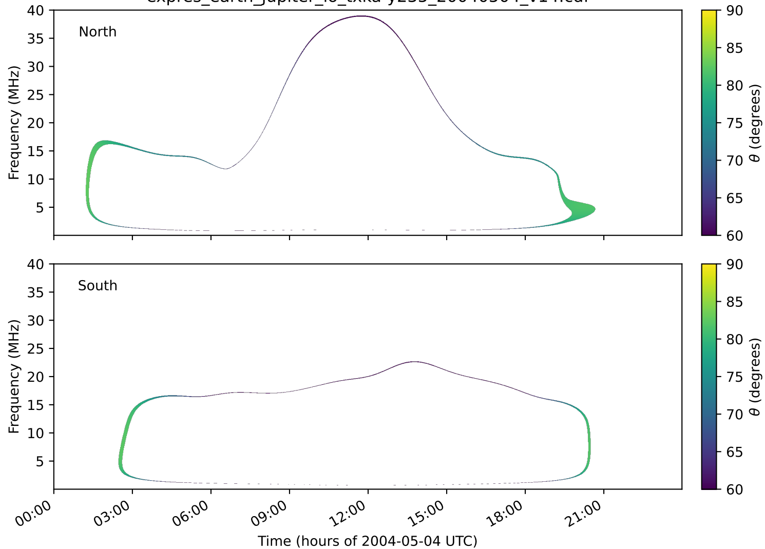
expres_earth_jupiter_io_txka-y235_20040504_v14.cdf
