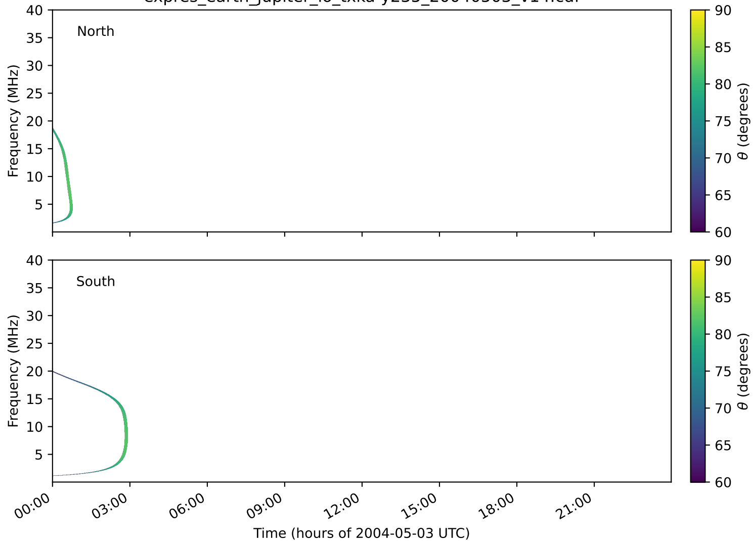
expres_earth_jupiter_io_txka-y235_20040503_v14.cdf
