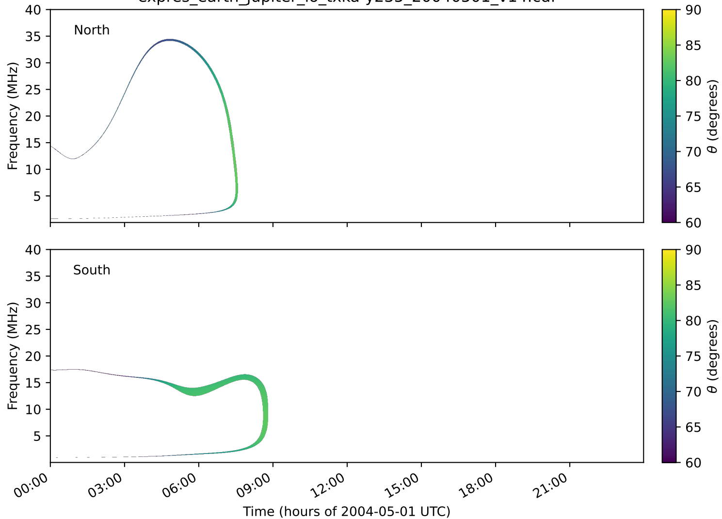
expres_earth_jupiter_io_txka-y235_20040501_v14.cdf
