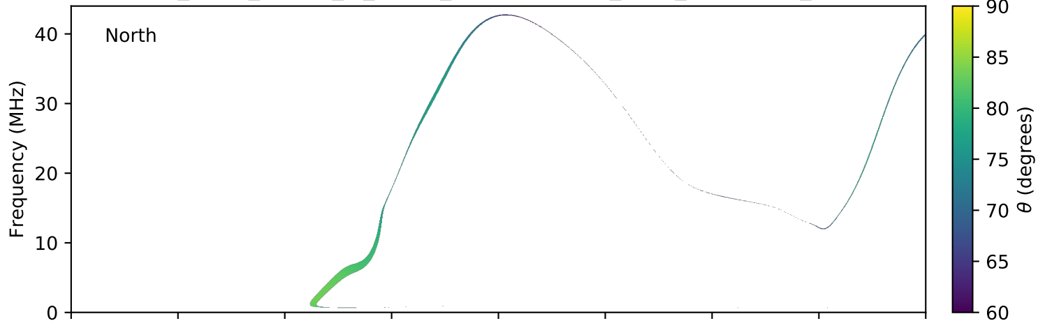
expres_earth_jupiter_io_jrm09_lossc-wid1deg_3kev_20040525_v11.cdf
