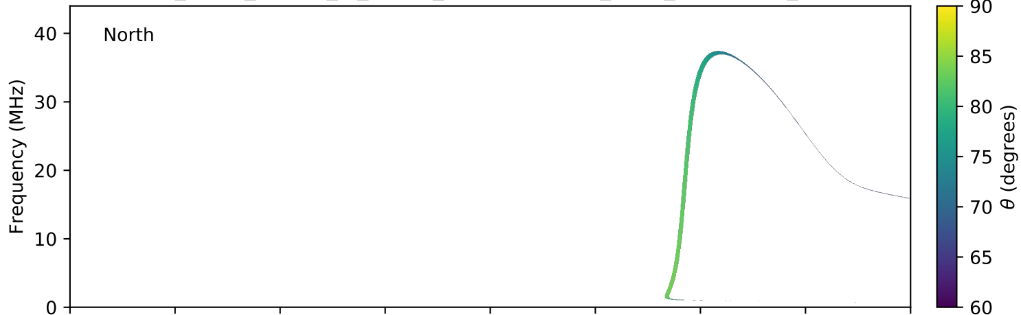
expres_earth_jupiter_io_jrm09_lossc-wid1deg_3kev_20040514_v11.cdf
