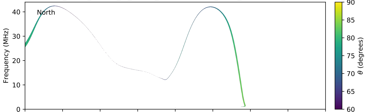
expres_earth_jupiter_io_jrm09_lossc-wid1deg_3kev_20040513_v11.cdf
