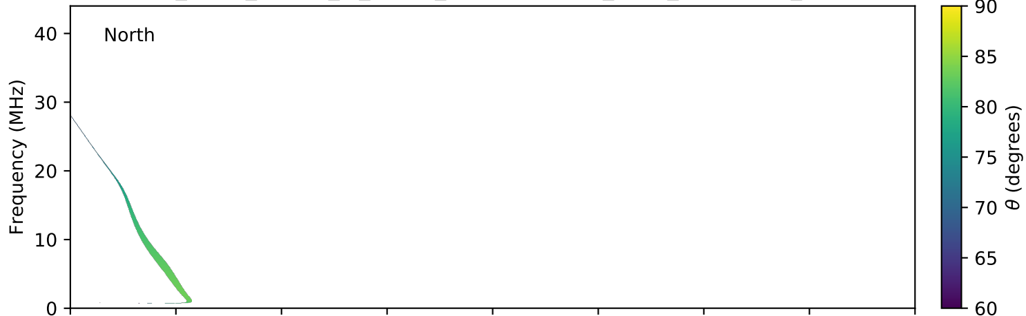
expres_earth_jupiter_io_jrm09_lossc-wid1deg_3kev_20040510_v11.cdf
