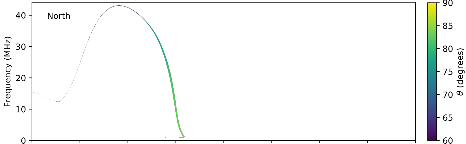
expres_earth_jupiter_io_jrm09_lossc-wid1deg_3kev_20040508_v11.cdf
