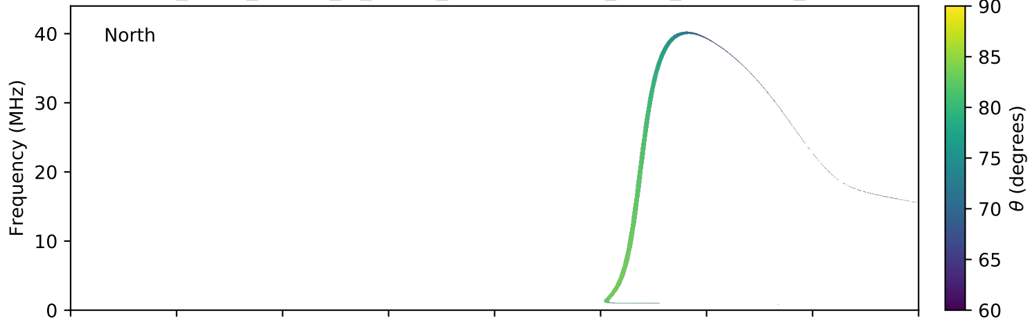
expres_earth_jupiter_io_jrm09_lossc-wid1deg_3kev_20040507_v11.cdf
