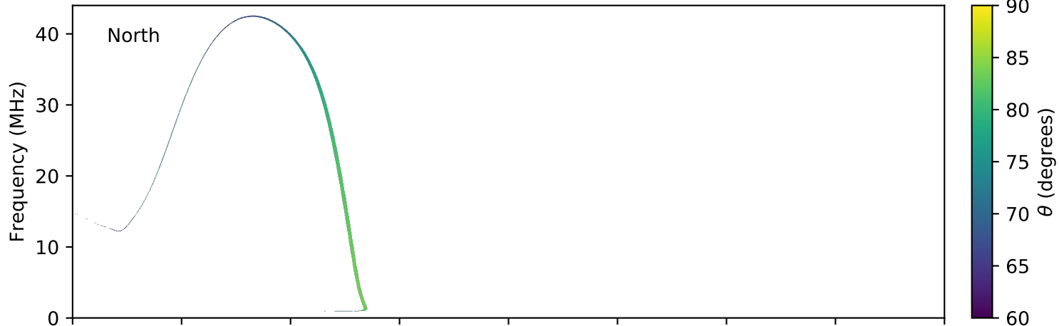
expres_earth_jupiter_io_jrm09_lossc-wid1deg_3kev_20040501_v11.cdf
