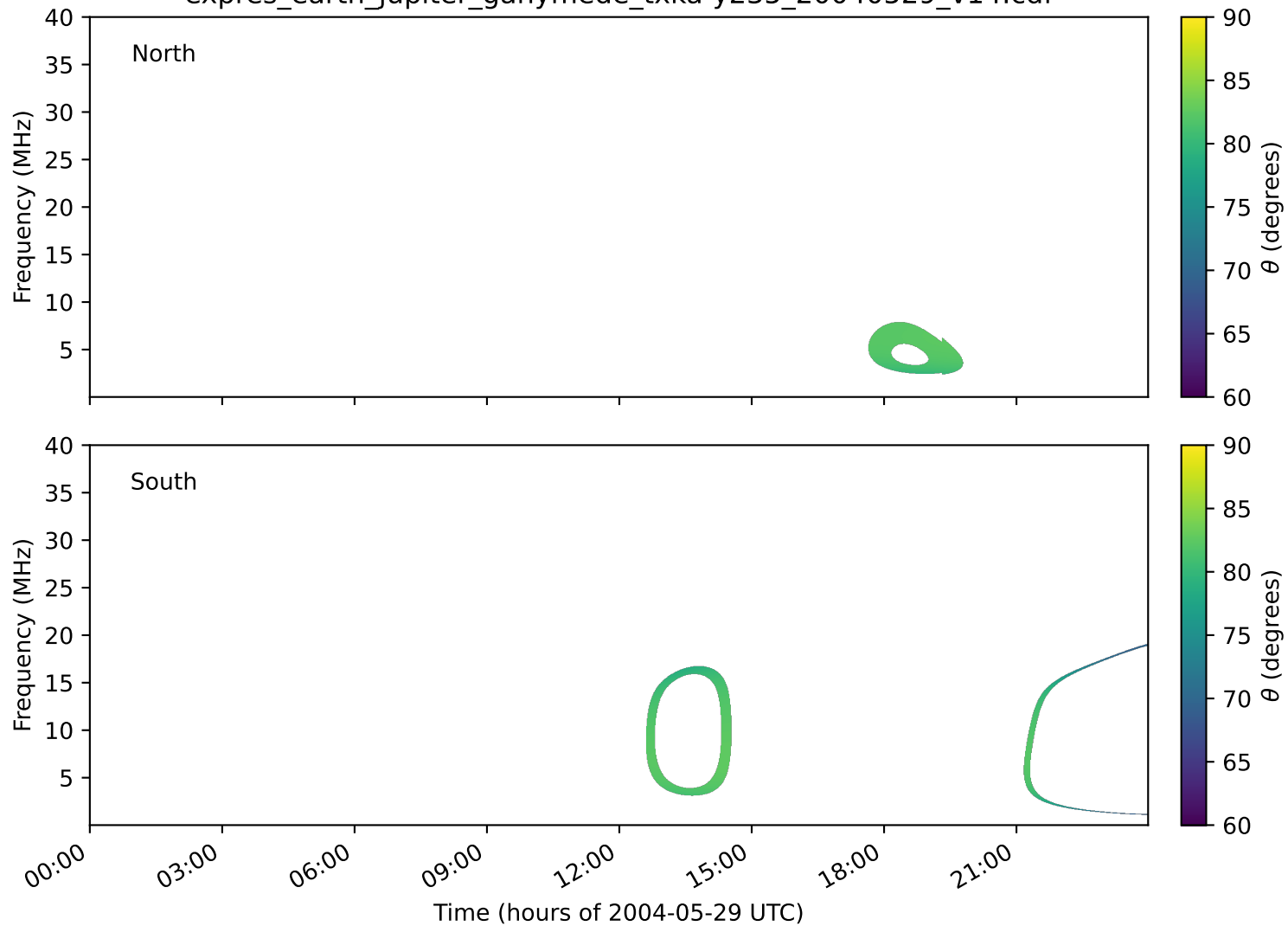
expres_earth_jupiter_ganymede_txka-y235_20040529_v14.cdf
