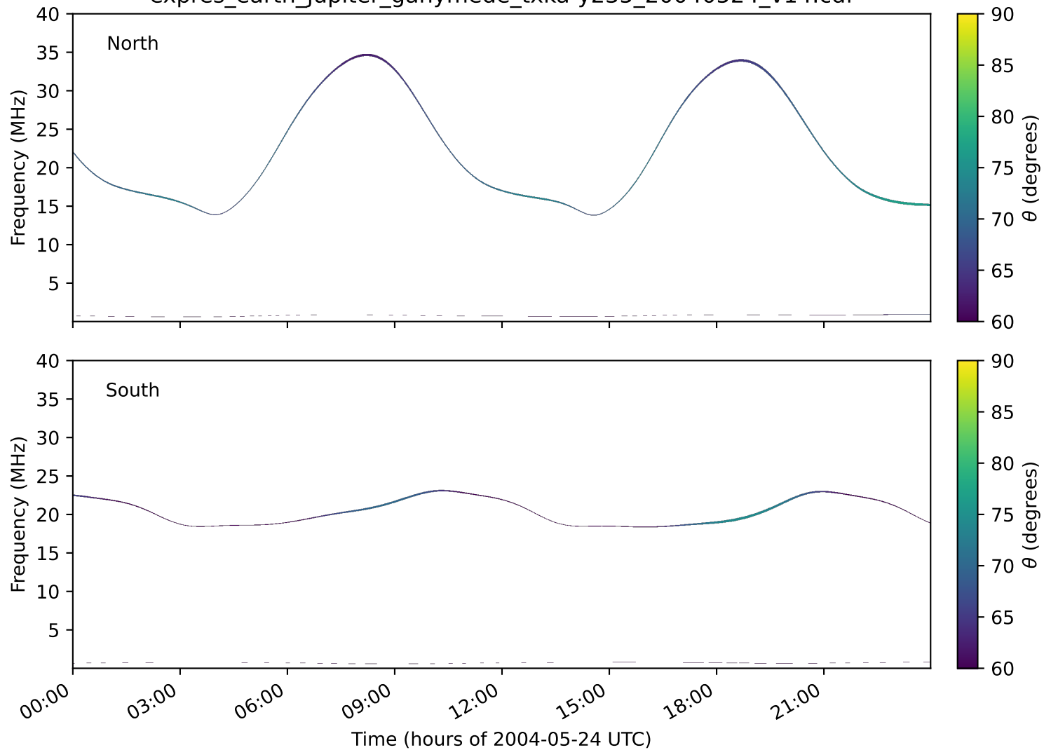
expres_earth_jupiter_ganymede_txka-y235_20040524_v14.cdf
