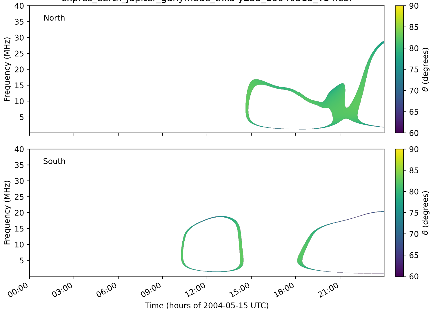
expres_earth_jupiter_ganymede_txka-y235_20040515_v14.cdf
