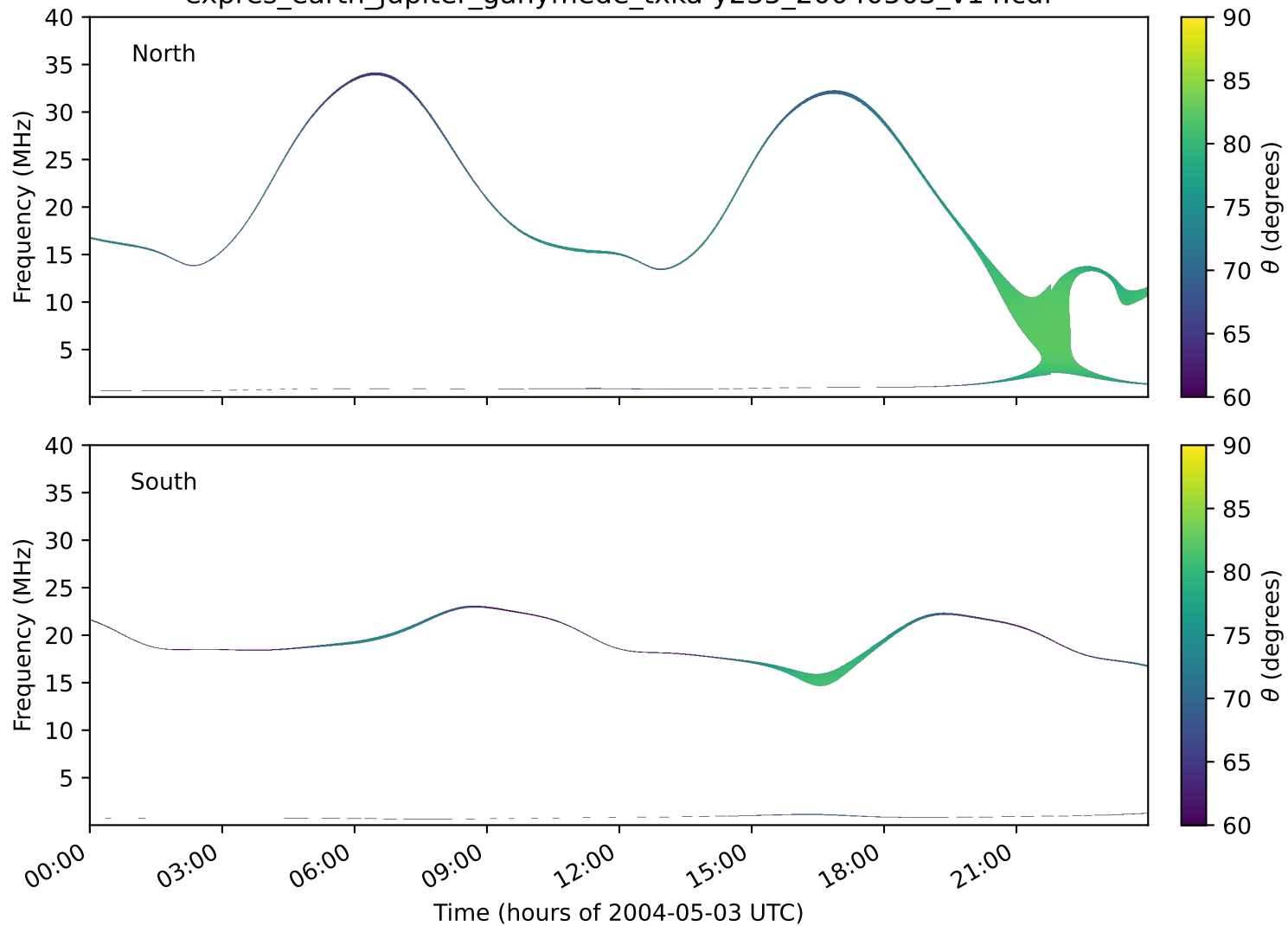
expres_earth_jupiter_ganymede_txka-y235_20040503_v14.cdf
