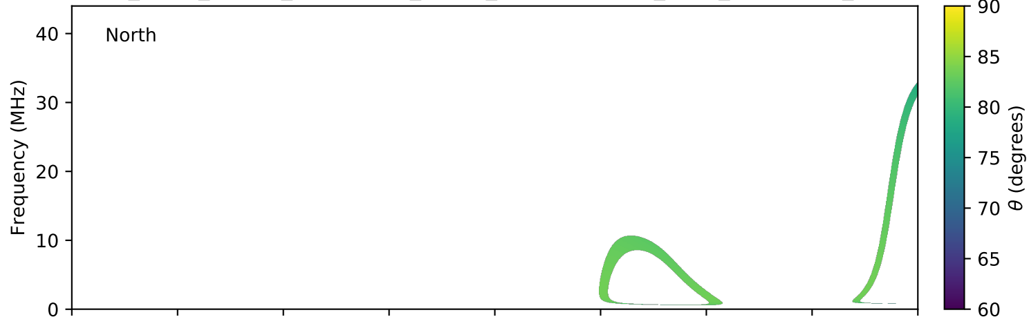
expres_earth_jupiter_ganymede_jrm09_lossc-wid1deg_3kev_20040515_v11.cdf
