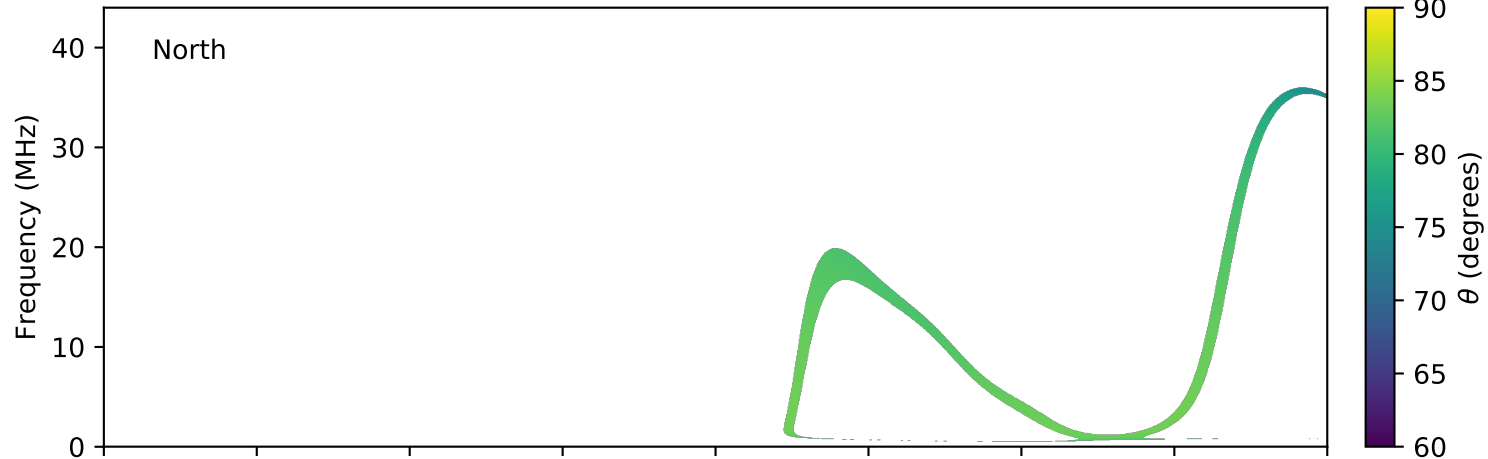
expres_earth_jupiter_ganymede_jrm09_lossc-wid1deg_3kev_20040508_v11.cdf
