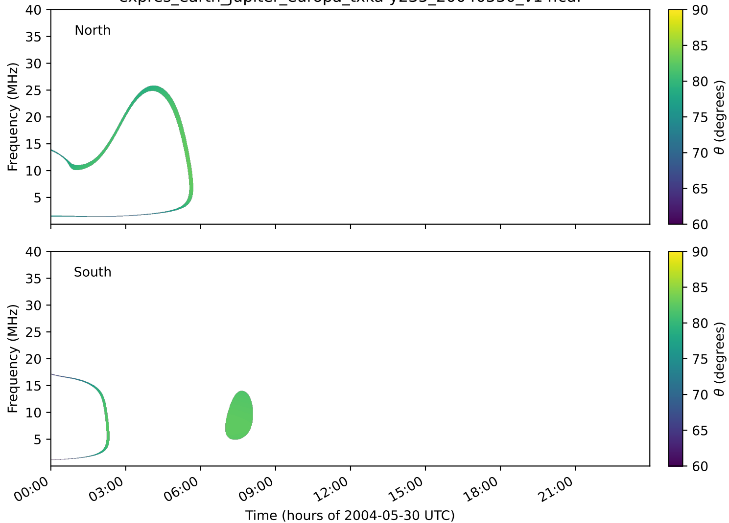
expres_earth_jupiter_europa_txka-y235_20040530_v14.cdf
