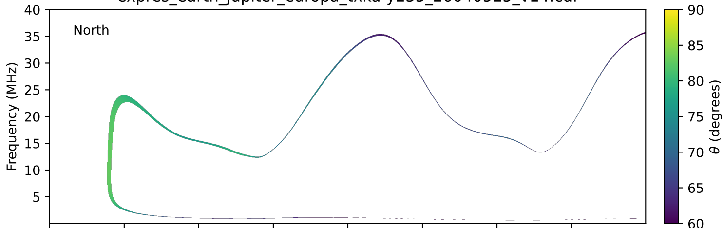
expres_earth_jupiter_europa_txka-y235_20040525_v14.cdf
