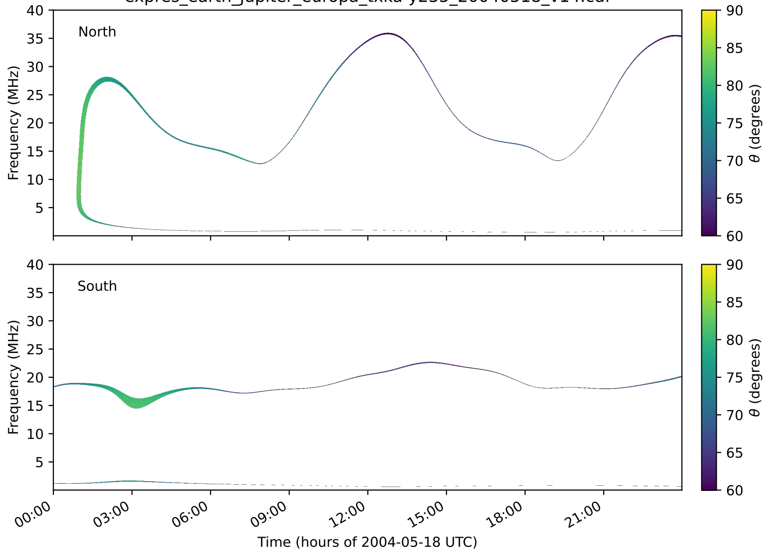
expres_earth_jupiter_europa_txka-y235_20040518_v14.cdf
