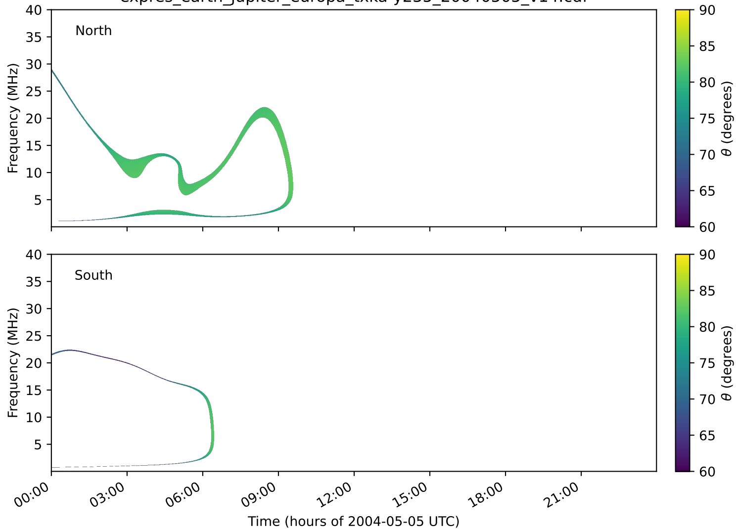
expres_earth_jupiter_europa_txka-y235_20040505_v14.cdf
