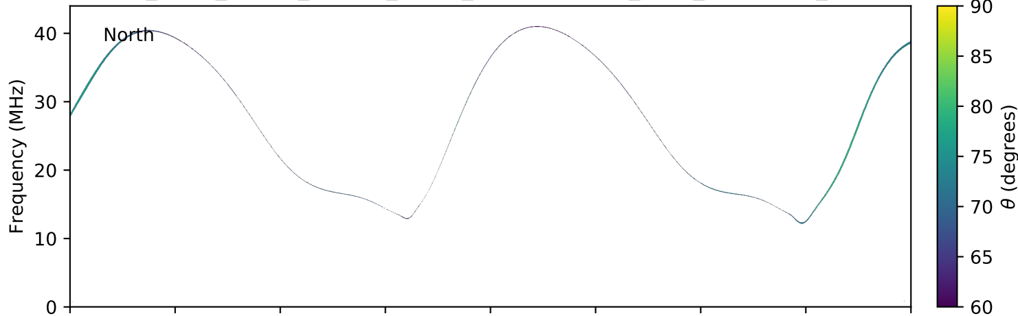
expres_earth_jupiter_europa_jrm09_lossc-wid1deg_3kev_20040531_v11.cdf
