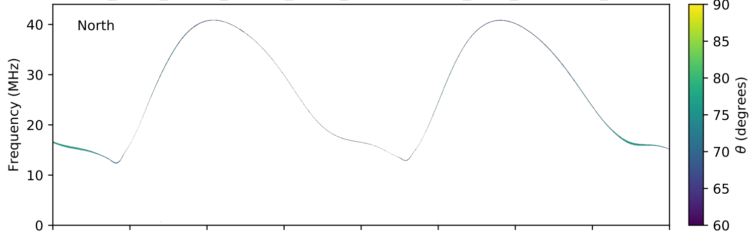
expres_earth_jupiter_europa_jrm09_lossc-wid1deg_3kev_20040529_v11.cdf
