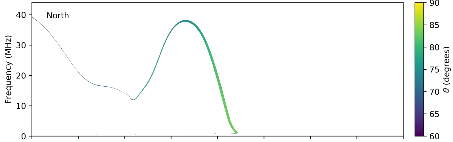
expres_earth_jupiter_europa_jrm09_lossc-wid1deg_3kev_20040519_v11.cdf
