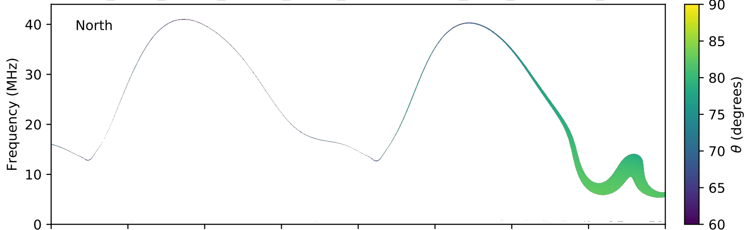
expres_earth_jupiter_europa_jrm09_lossc-wid1deg_3kev_20040515_v11.cdf
