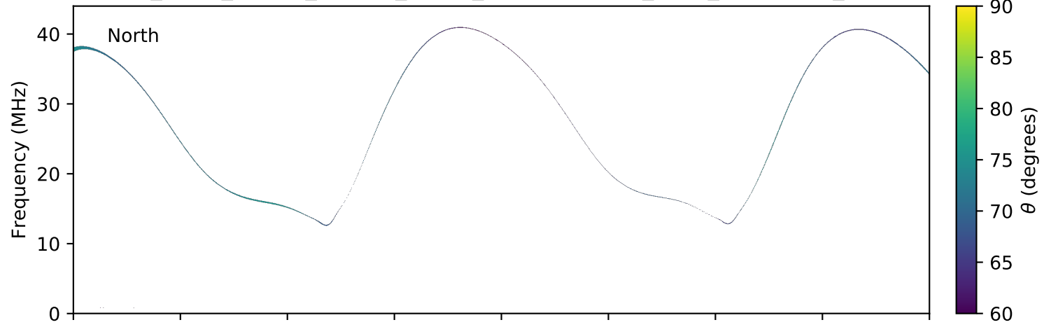
expres_earth_jupiter_europa_jrm09_lossc-wid1deg_3kev_20040504_v11.cdf
