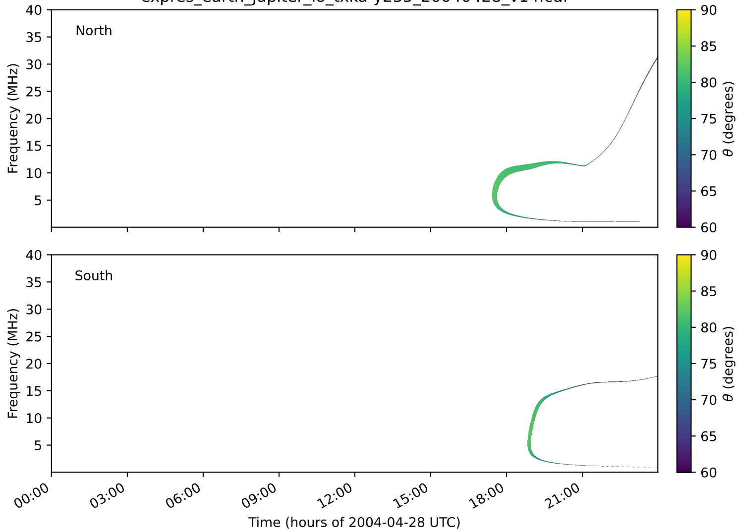
expres_earth_jupiter_io_txka-y235_20040428_v14.cdf
