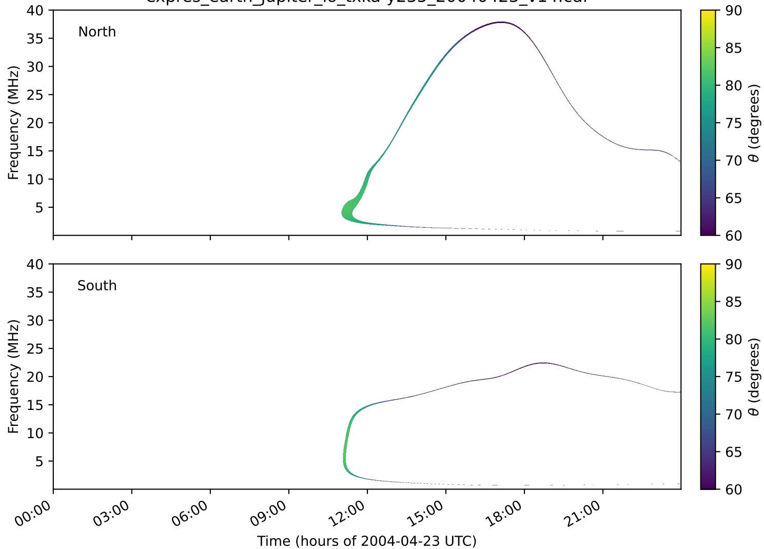
expres_earth_jupiter_io_txka-y235_20040423_v14.cdf
