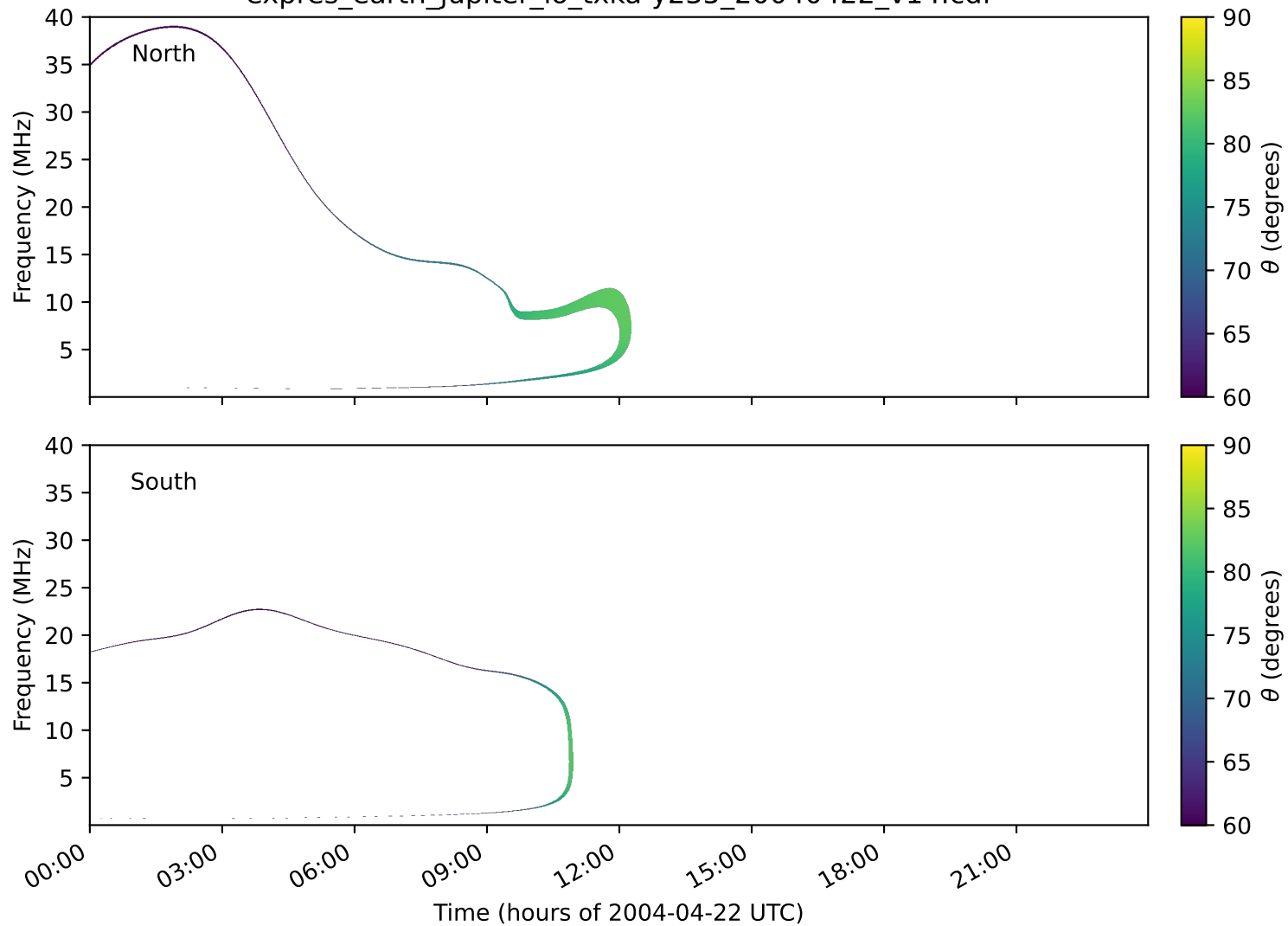
expres_earth_jupiter_io_txka-y235_20040422_v14.cdf
