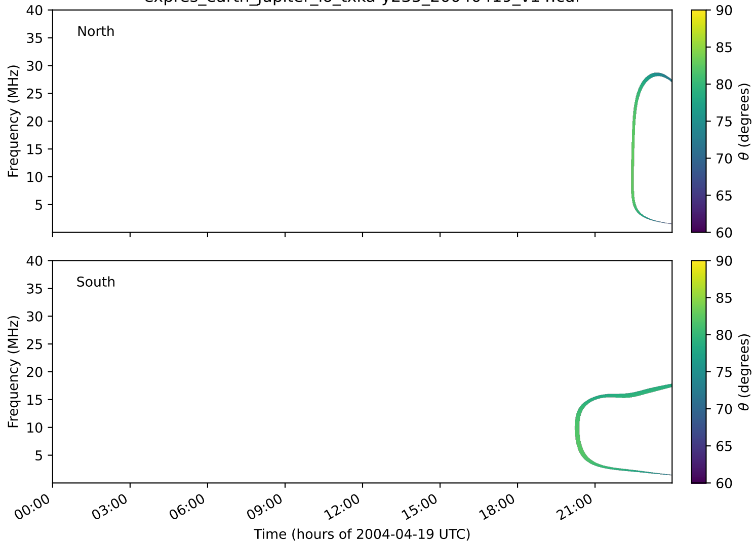
expres_earth_jupiter_io_txka-y235_20040419_v14.cdf
