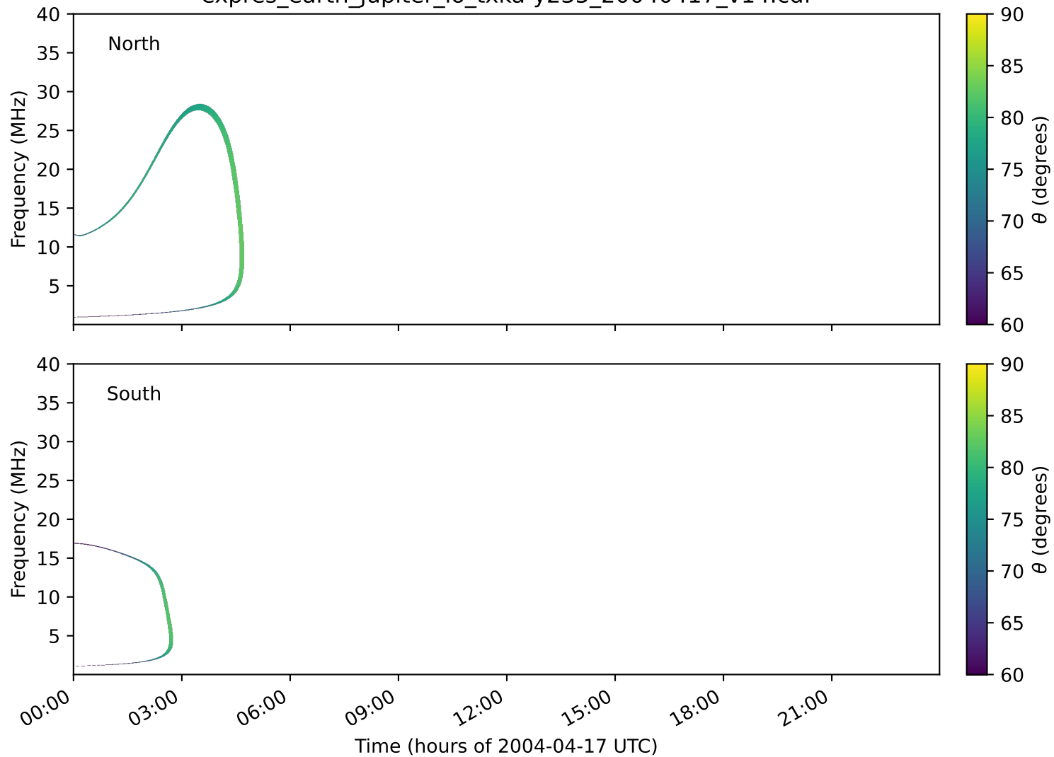
expres_earth_jupiter_io_txka-y235_20040417_v14.cdf
