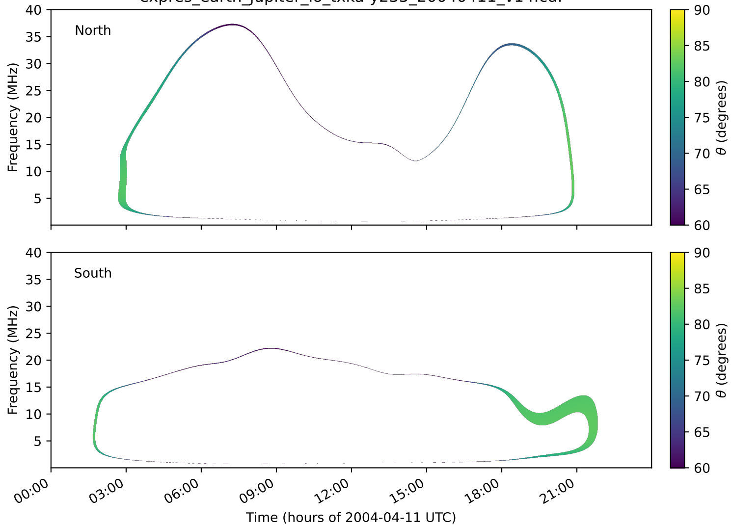
expres_earth_jupiter_io_txka-y235_20040411_v14.cdf
